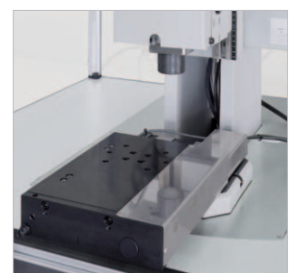
SCHMIDT® Slide Table ST 150P, pneumatic operating mode
